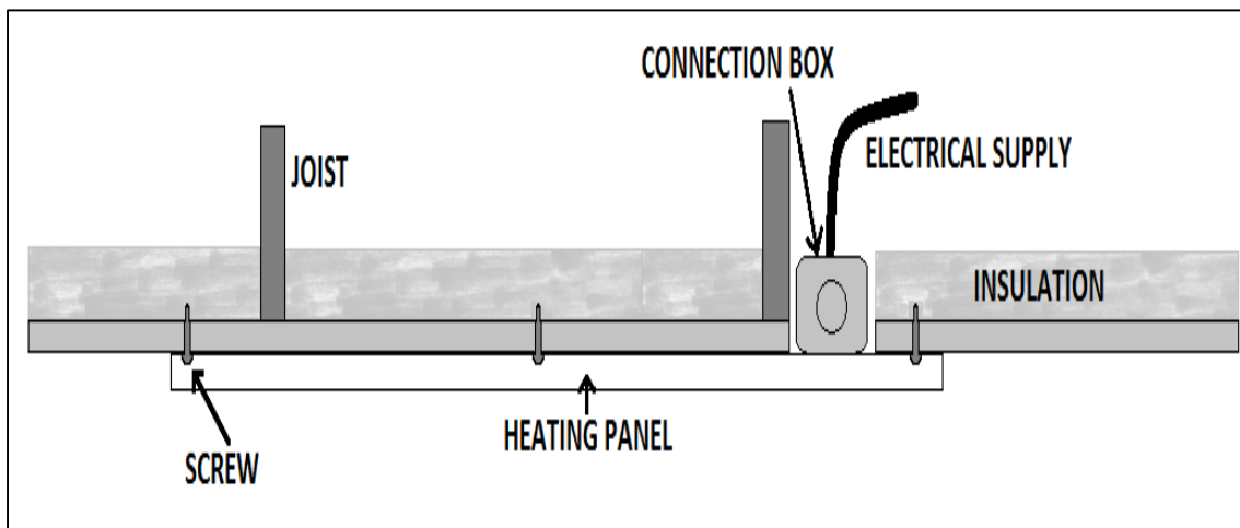
Figure 1 – Surface Mounting
